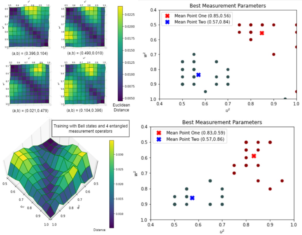
Figure 14: Bell and X states best measurements and points cluster
