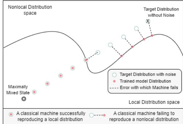
Figure 16: Adding noise to nonlocal distribution
