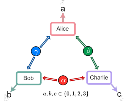
Figure 21: The two best choice of measurements
