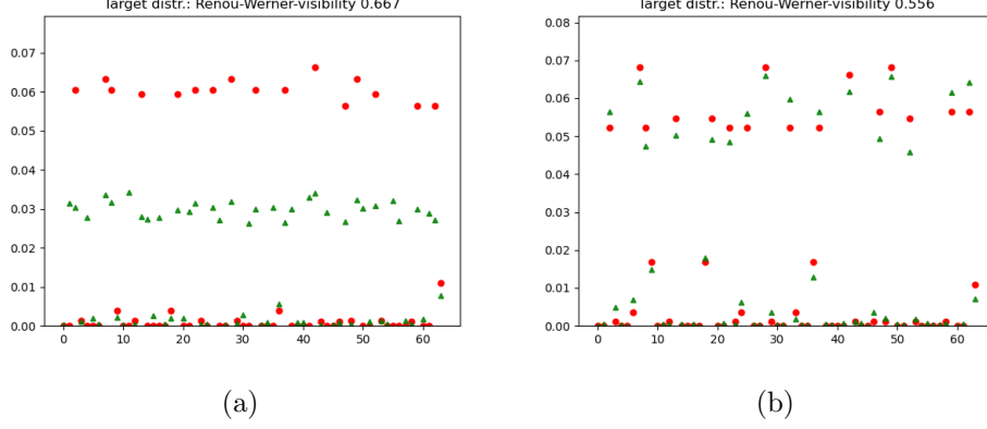
Figure 22: The distributions show that only a few elements of the 64 probability distributions are responsible for nonlocal behavior
