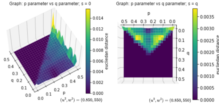
Figure 19: p, q vs euclidean distances
