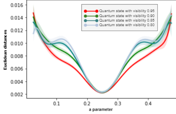
Figure 17: Euclidean distances for varying noise visibilities
