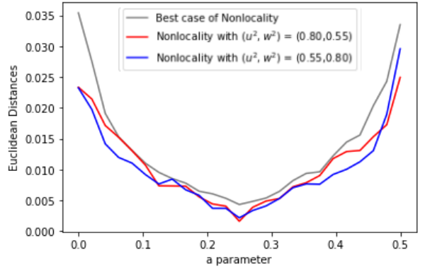
Figure 15: The two best choice of measurements
